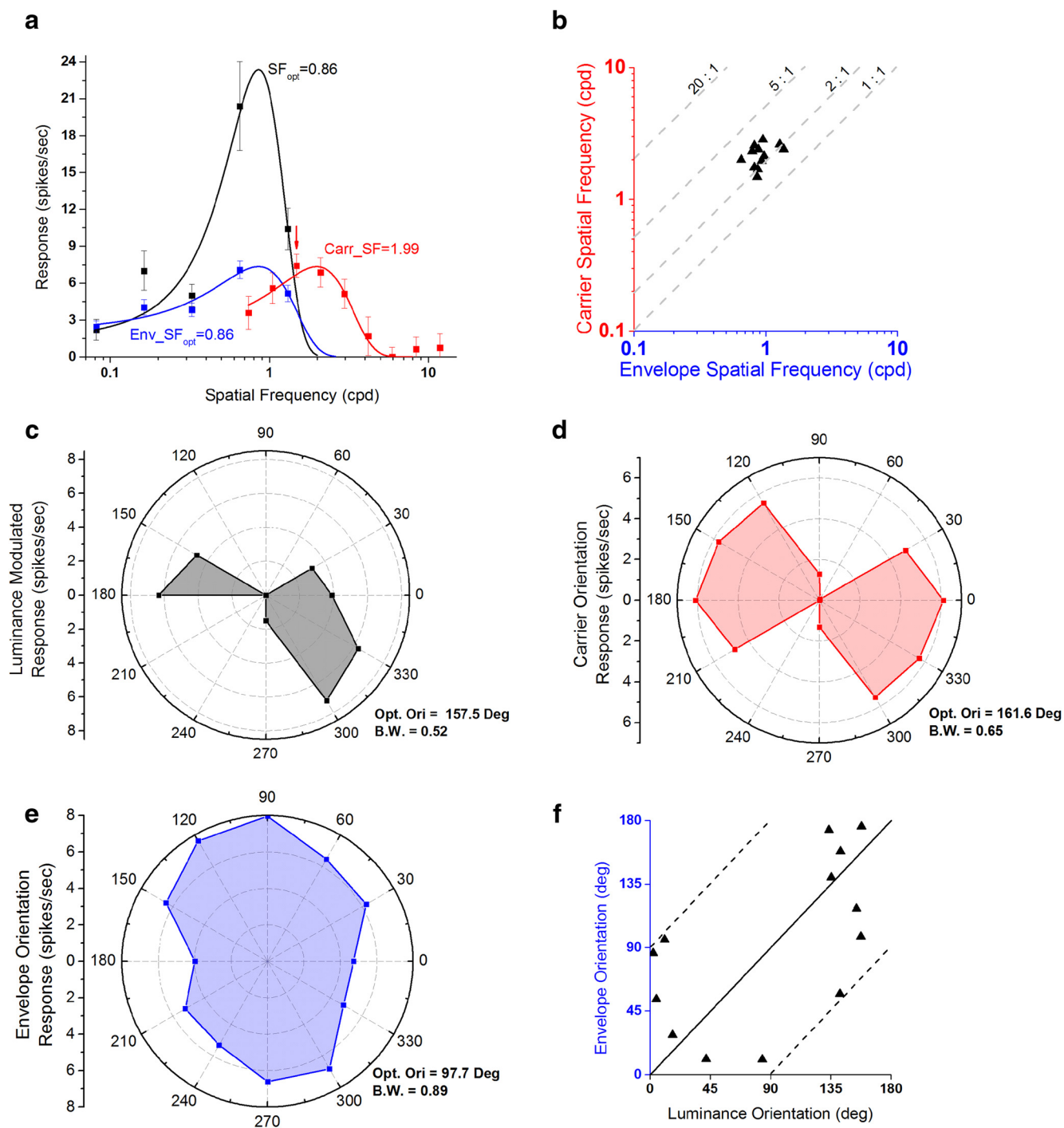
Figure 7. Tuning properties of response to CM gratings having carrier SFs inside a neuron's frequency-selective range for luminance gratings. a , Example of SF responses for one neuron. The SF tuning for luminance gratings is plotted in black. The CM tuning properties of this neuron were measured with a carrier SF (red arrow) that was inside the neuron's frequency-selective range for luminance gratings. The SF tuning for envelope responses is plotted in blue. Error bars indicate \pm SE . b , Scatter plot of results from several similarly tested neurons. Each point indicates one neuron's carrier SF plotted against its optimal envelope SF. All points are distributed around a 2:1 ratio line (hence we refer to these as 2:1 neurons; N = 12 ). c–e , Orientation polar plots for the same neuron shown in a , for luminance gratings ( c , black), CM carriers ( d , red), and CM envelopes ( e , blue). Distance from the origin represents magnitude of response and polar angle represents orientation. Optimal orientation (Opt. Ori) and bandwidth (B.W.) of each tuning curve are given at bottom-right of the plot. f , Scatter plot of 2:1 neurons' optimal envelope orientations plotted against their optimal luminance orientations ( N = 13 ). Spontaneous activity was removed in tuning curve plots ( a , c–e ).
