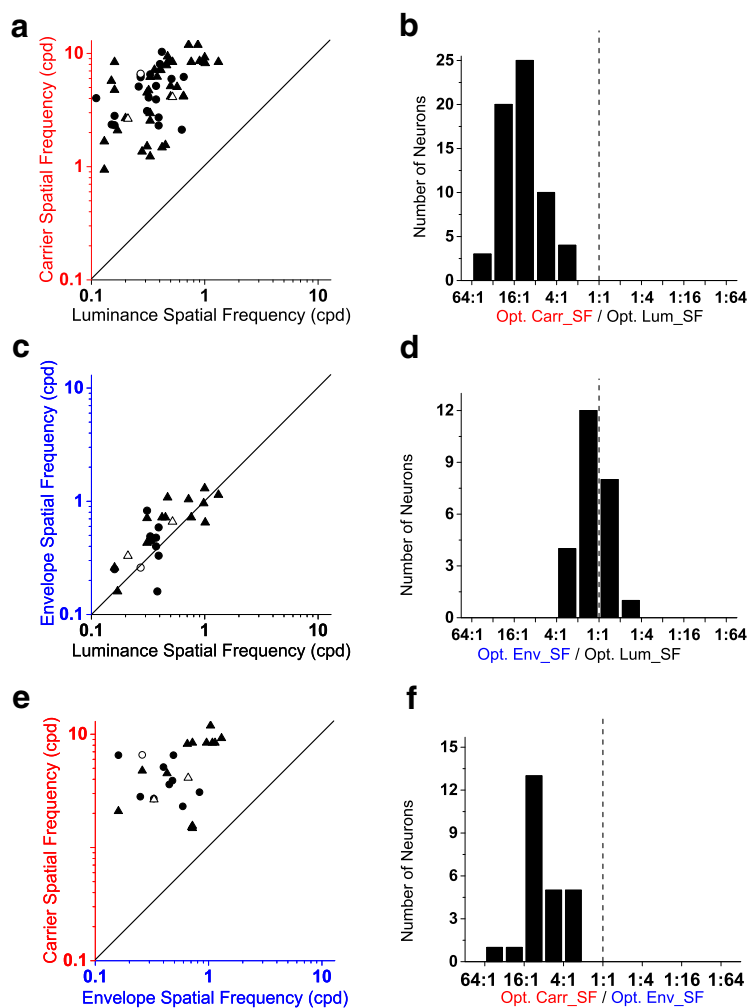
Figure 3. Optimal SFs for CM gratings and luminance gratings. a, c, e , Scatter plots of optimal SFs of sampled neurons. Each point represents one neuron's optimal SF for CM carriers plotted against that for luminance gratings ( a ), envelope plotted against luminance ( c ), and carrier plotted against envelope ( e ). Solid lines depict the unity ratio. b, d, f , Histograms of ratios for data shown in a, c , and e . b , Ratios of neurons' optimal carrier-to-luminance SF values (median, 12.8:1). d , Ratios of neurons' optimal envelope-to-luminance SF. The ratios were \sim 1:1 , indicating that a neuron's optimal envelope SF was similar to its optimal luminance SF (median, 1.32:1). f , Ratios of neurons' optimal carrier-to-envelope SF (median, 8.21:1). Due to limitations of recording stability, the envelope tuning properties were only measured in a subset of CM neurons. Thus there are 62 pairs shown in a and b , and 25 pairs in c–f . Circles indicate neurons with simple-type responses (21 in a , 10 in c and e ). Triangles indicate neurons with complex-type responses (41 in a , 15 in c and e ). Open symbols indicate the three example neurons shown in Figure 2.
